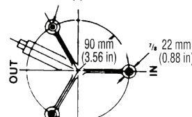
BOTTOM VIEW OF 38.1 mm (1.50 in) MAIN CASE
